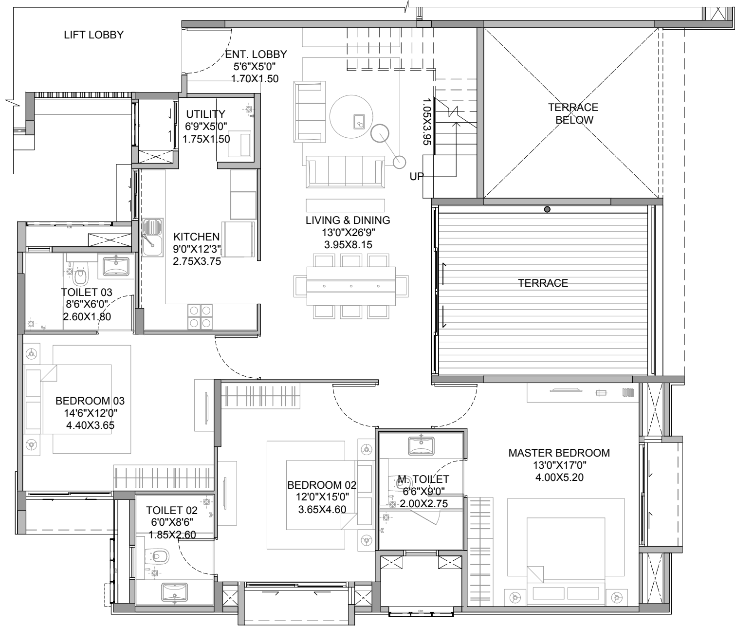
LOWER LEVEL PLAN
