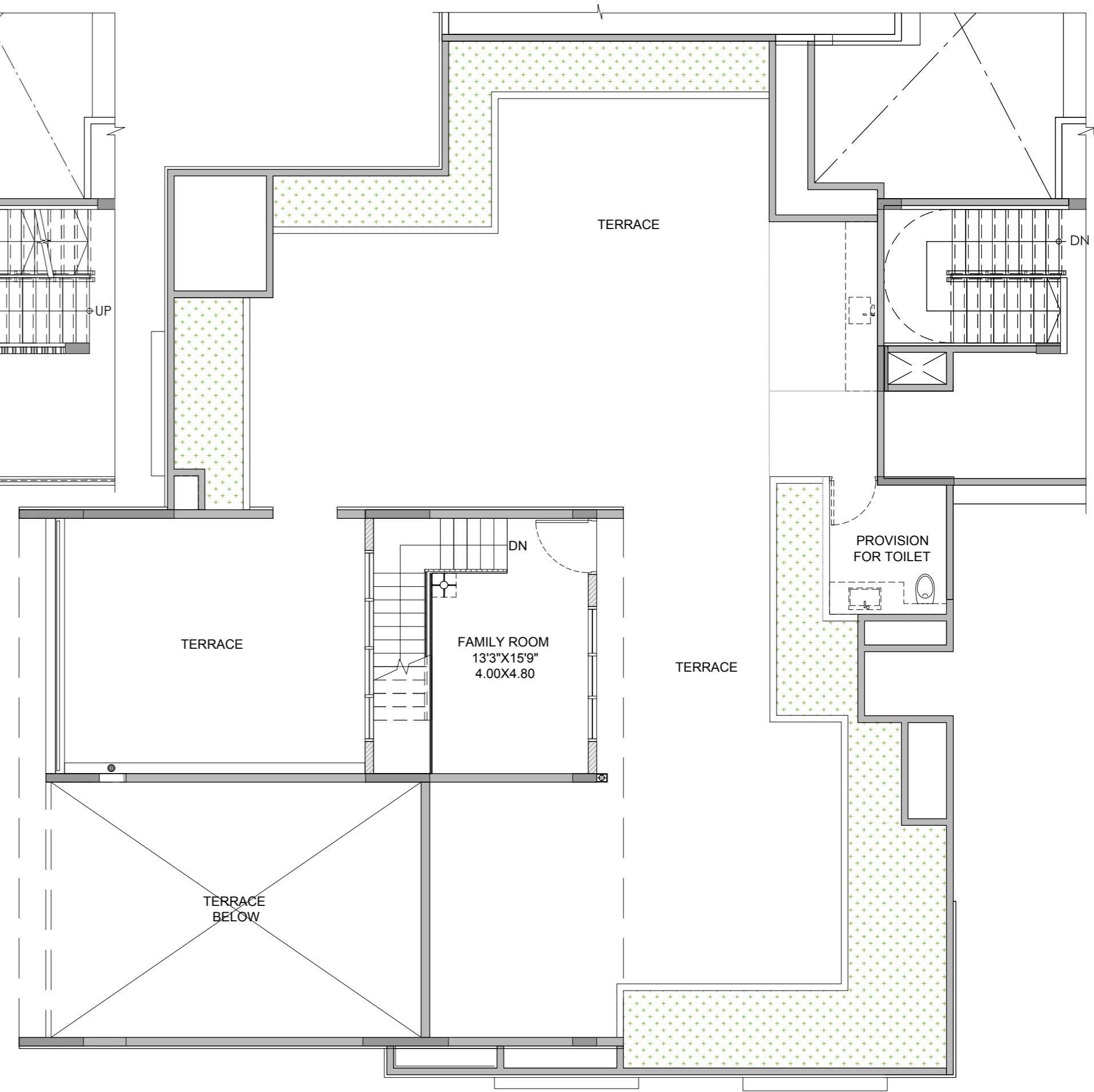
UPPER LEVEL PLAN
